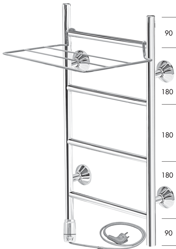
RKES-720-400 RKES-720-502
